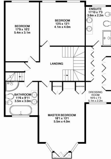
1ST FLOOR APPROX. FLOOR AREA 1148 SQ. FT. (106.7 SQ. M.)
