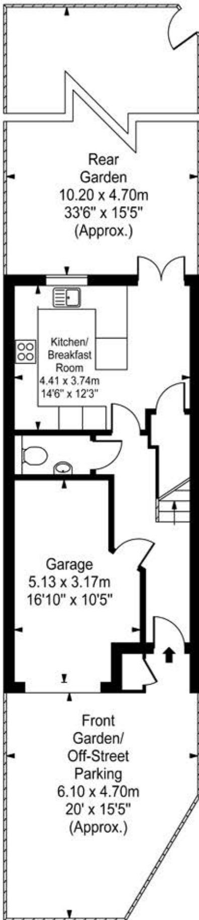
Ground Floor
